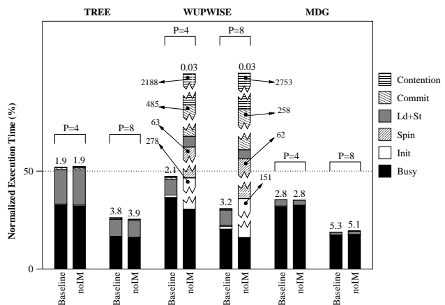
Figure 8: Normalized execution time breakdown for Baseline with and without the IM data structure optimization. In all cases we use the best window size from Figure 5. Results are shown for 4 and 8 processors ( P ). Note that the bars for WUPWISE noIM are truncated and the height of the bars are bigger than shown. The values of these truncated sections are shown in the figure. The numbers on top of the bars are the speedups relative to sequential execution.
